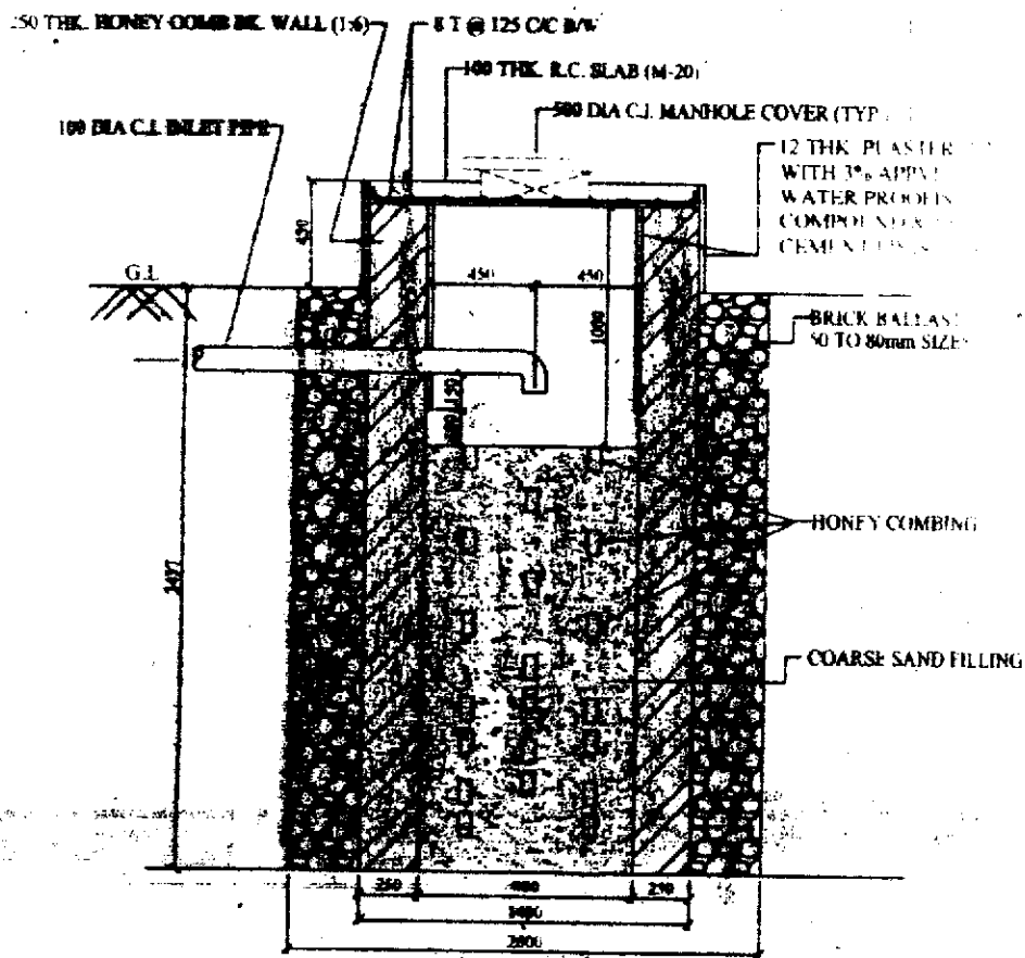
SECTION - ZZ
